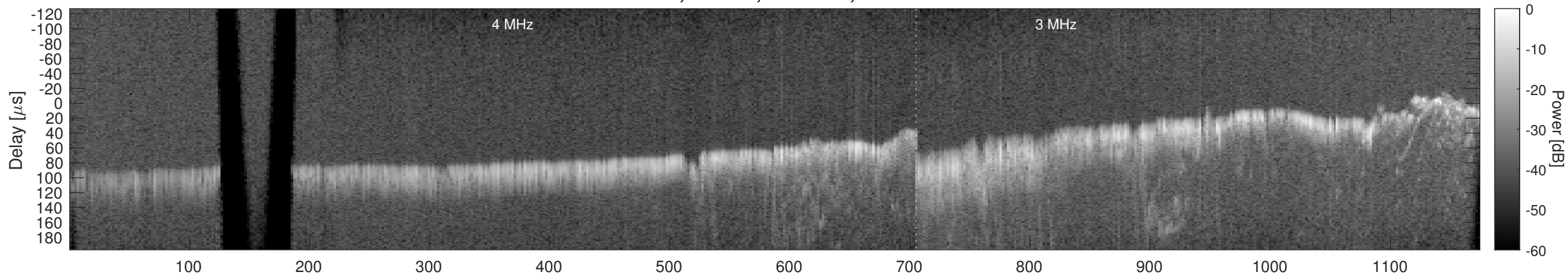
Orbit 15614, Window, Channel 2, Chapman
