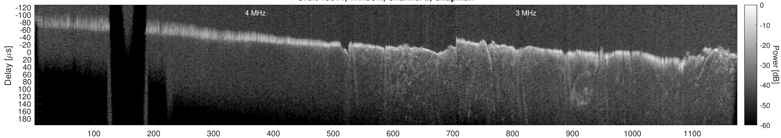
Orbit 15614, Window, Channel 2, Optimized
