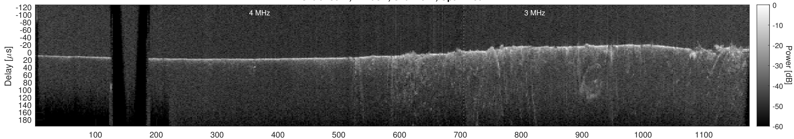
Orbit 15614, Cluttergram
