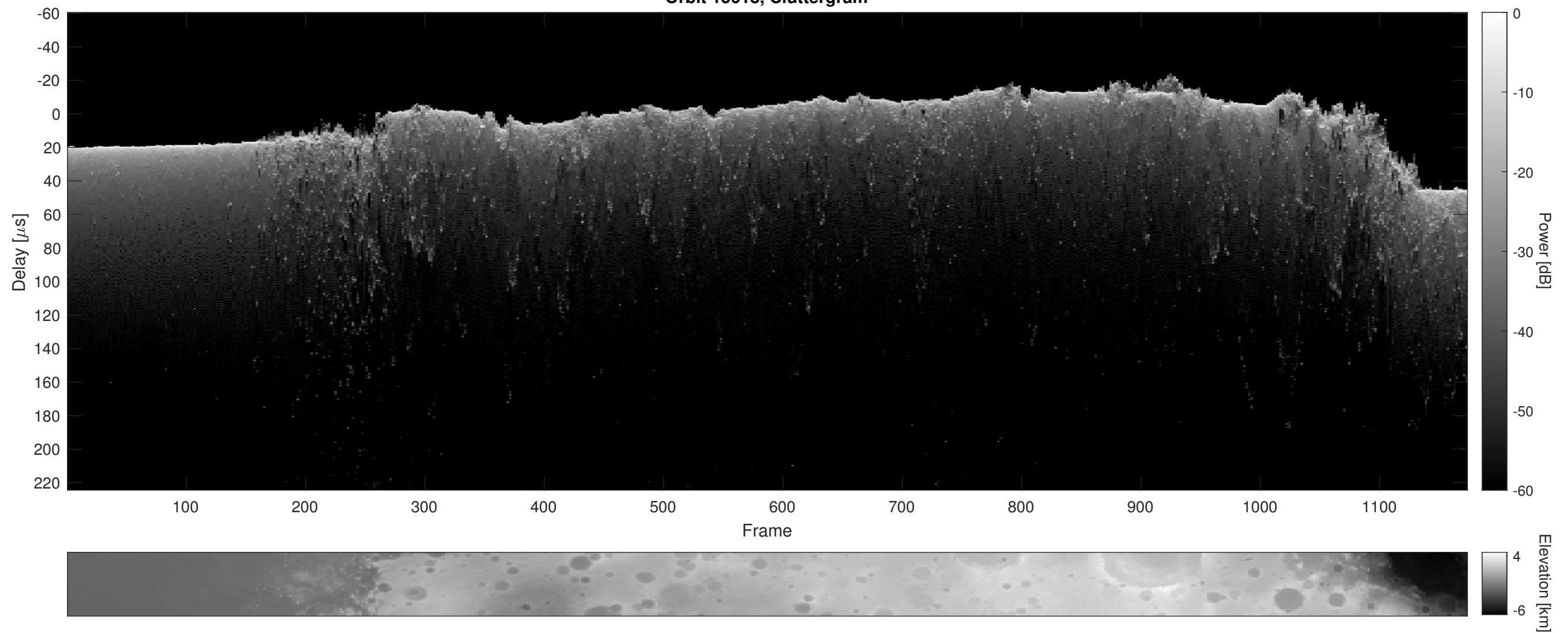
Orbit 15618, Cluttergram
