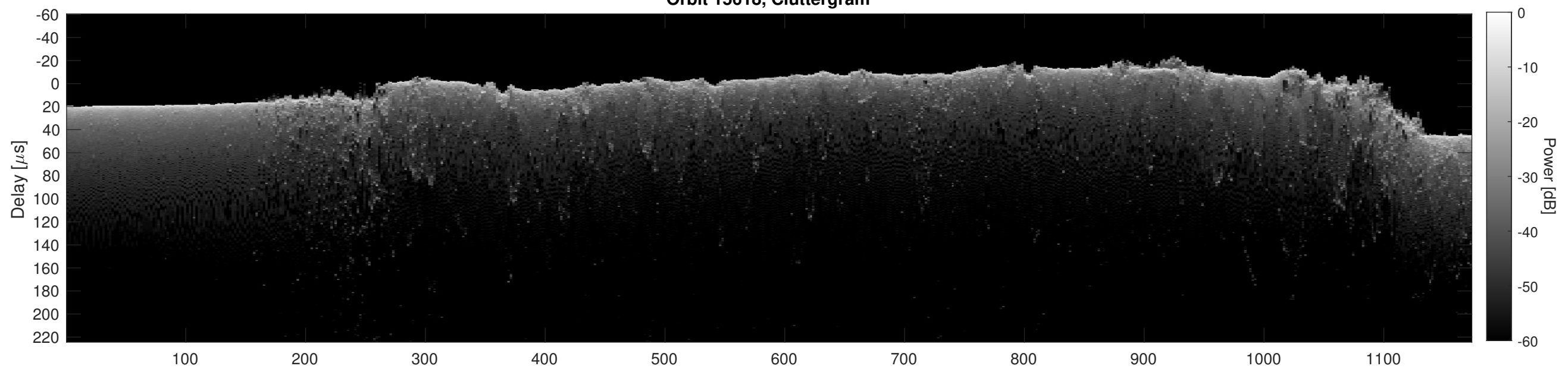
Orbit 15618, Cluttergram
