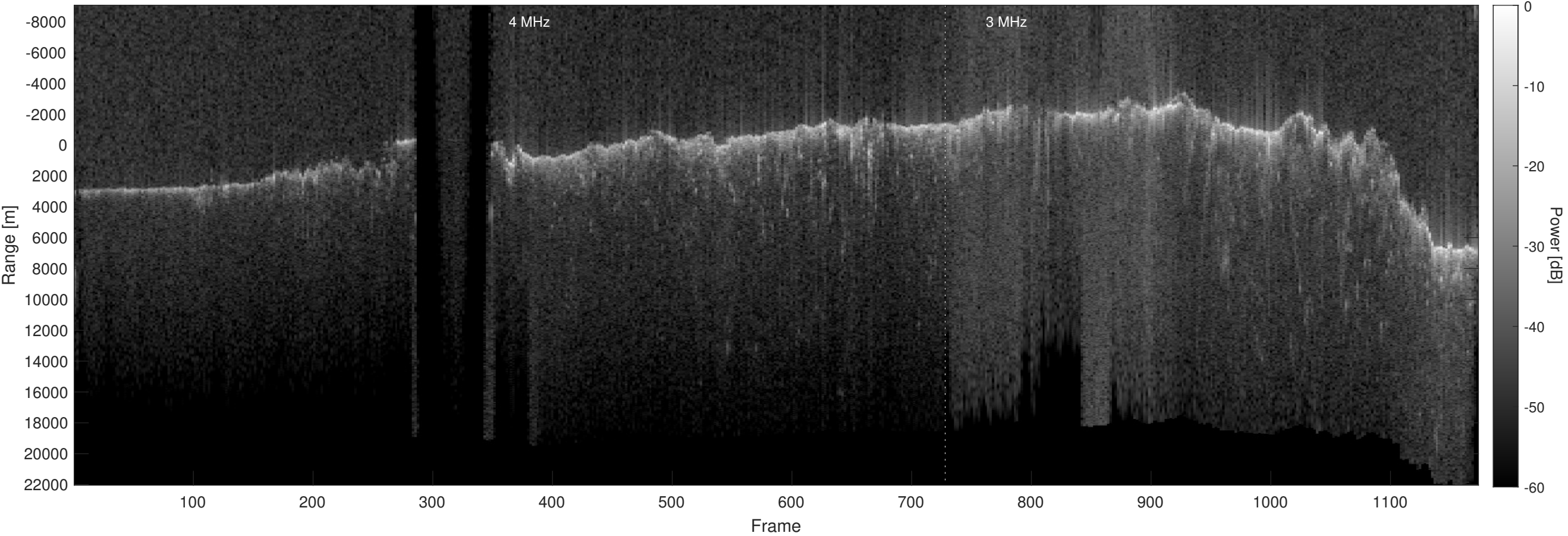
Orbit 15618, Optimized, No Window, Depth-Corrected, Channel 2
