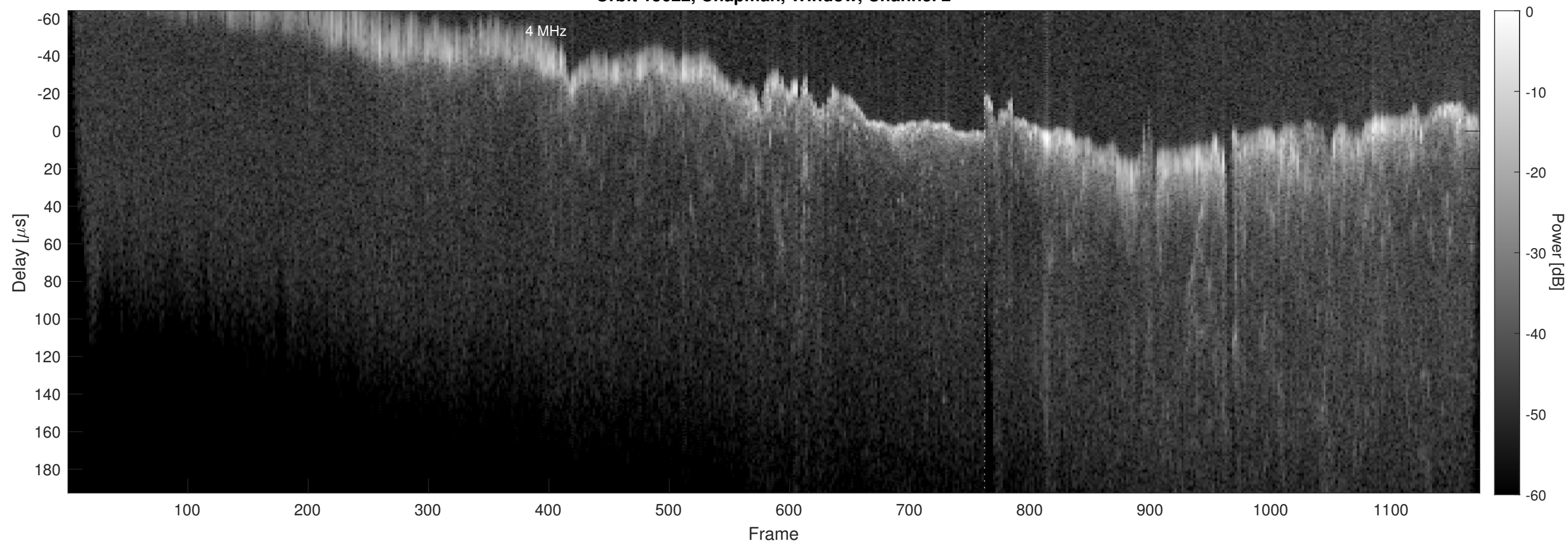
Orbit 15622, Chapman, Window, Channel 2
