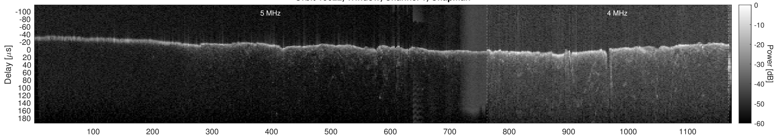
Orbit 15622, Window, Channel 1, Optimized
