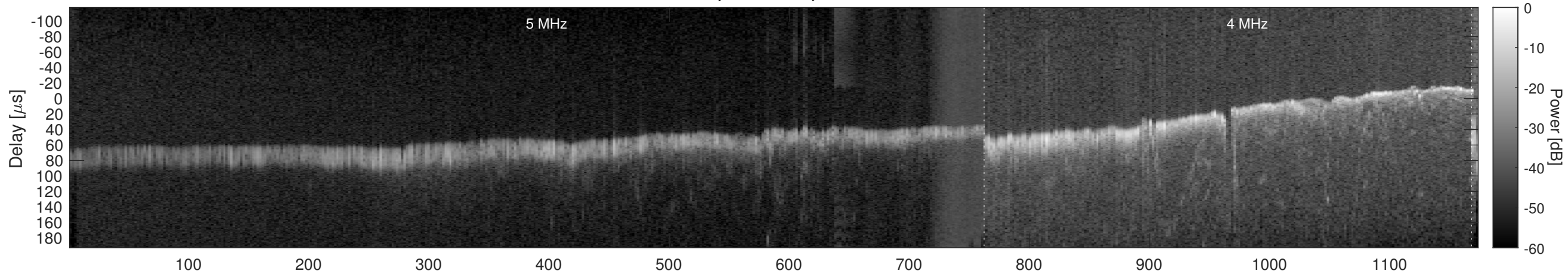
Orbit 15622, Window, Channel 1, Chapman
