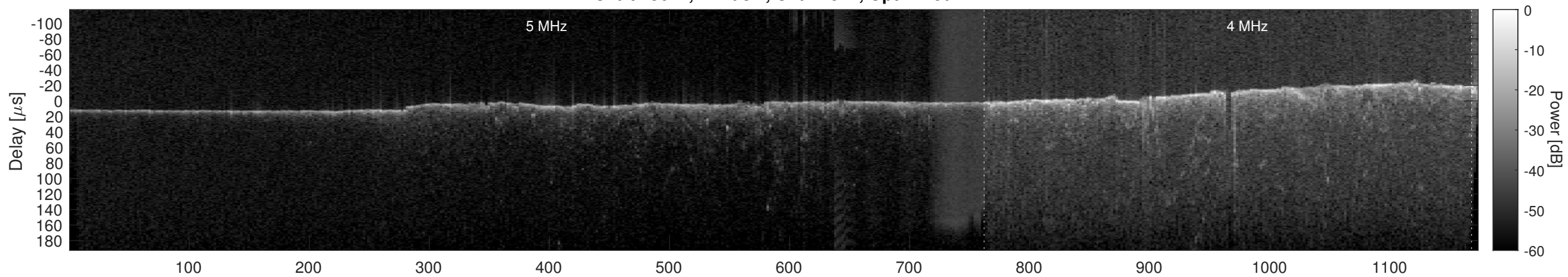
Orbit 15622, Cluttergram
