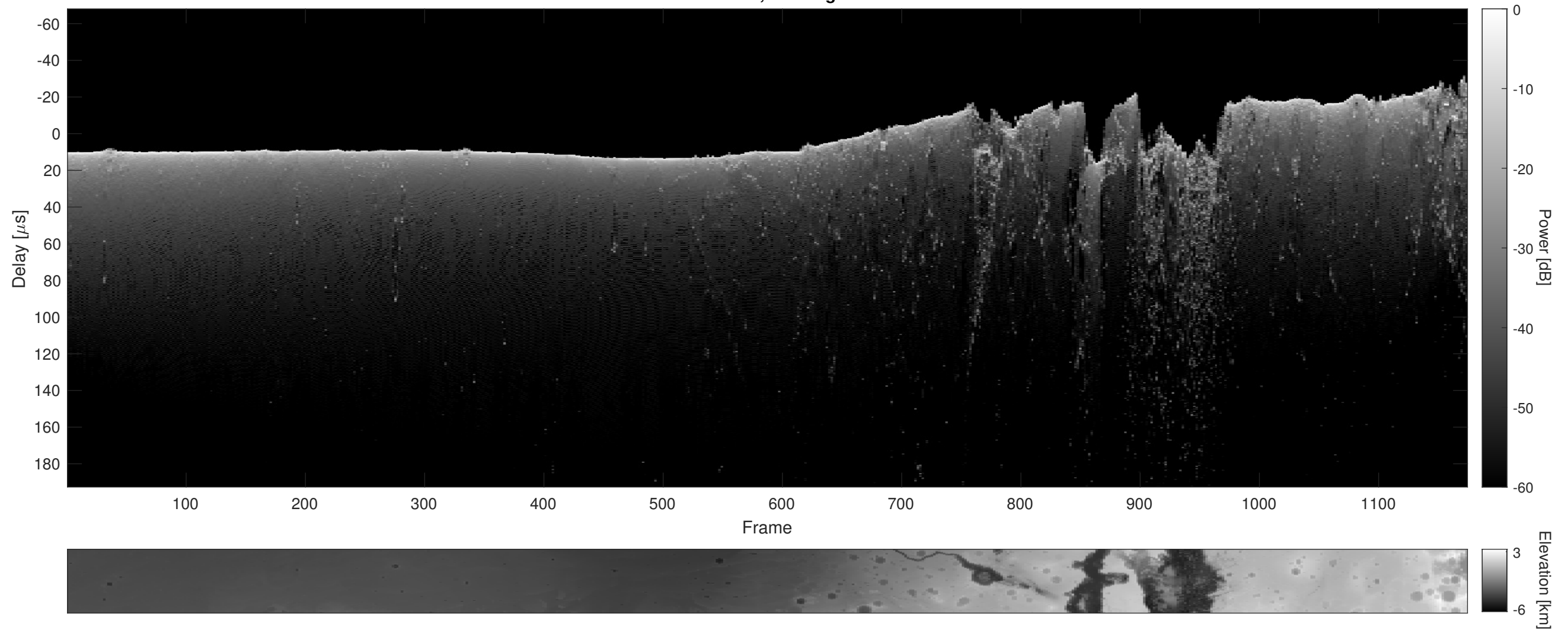
Orbit 15626, Cluttergram
