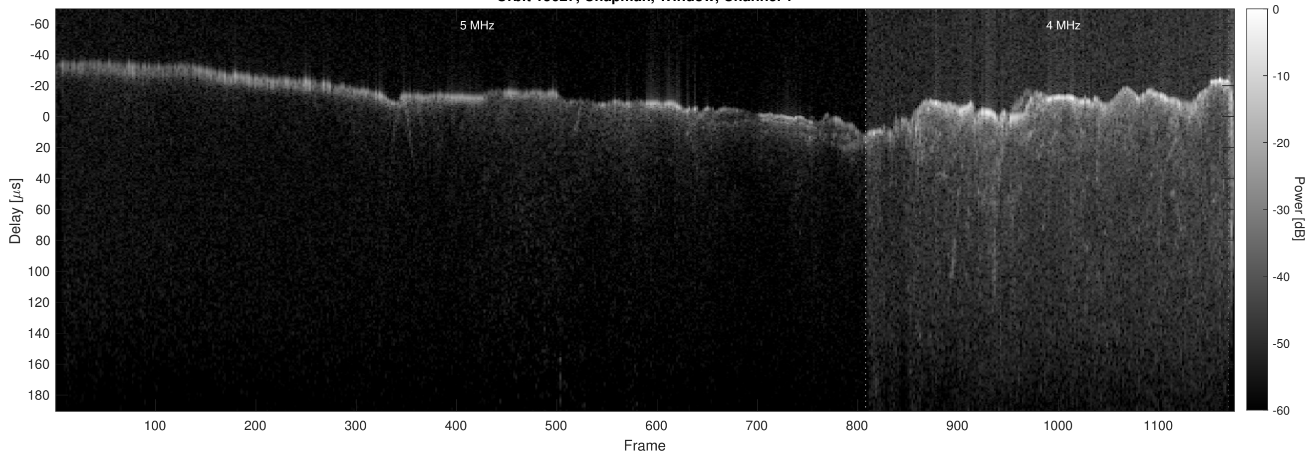
Orbit 15627, Chapman, Window, Channel 2
