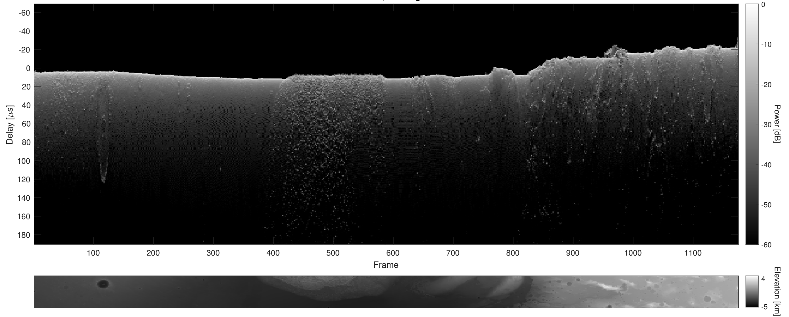
Orbit 15627, Cluttergram
