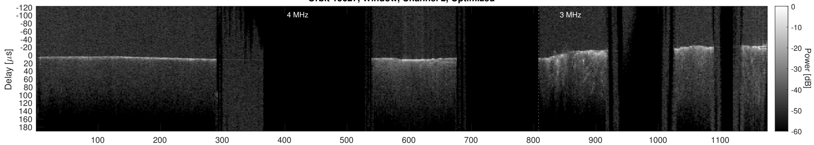
Orbit 15627, Cluttergram
