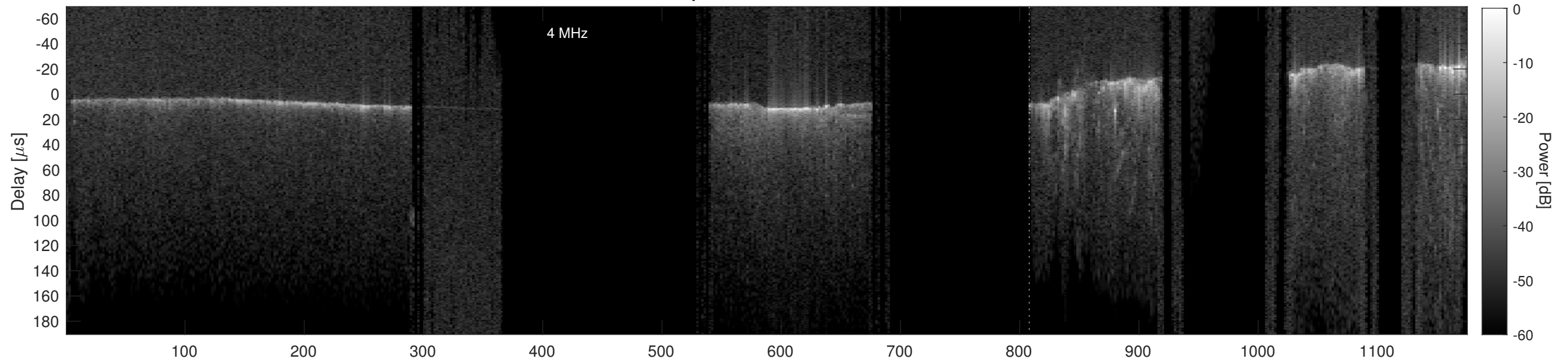
Orbit 15627, Cluttergram
