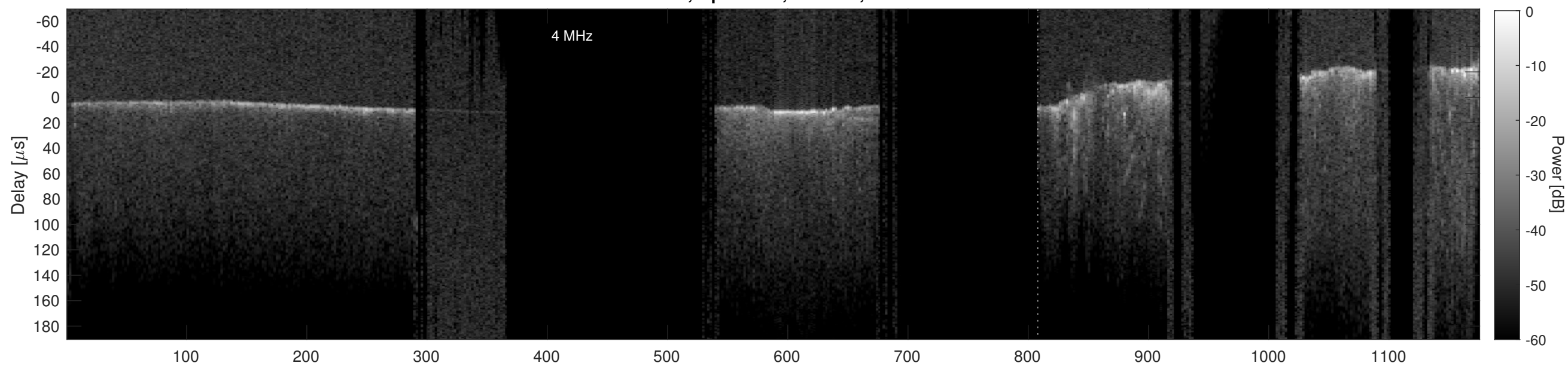
Orbit 15627, Cluttergram
