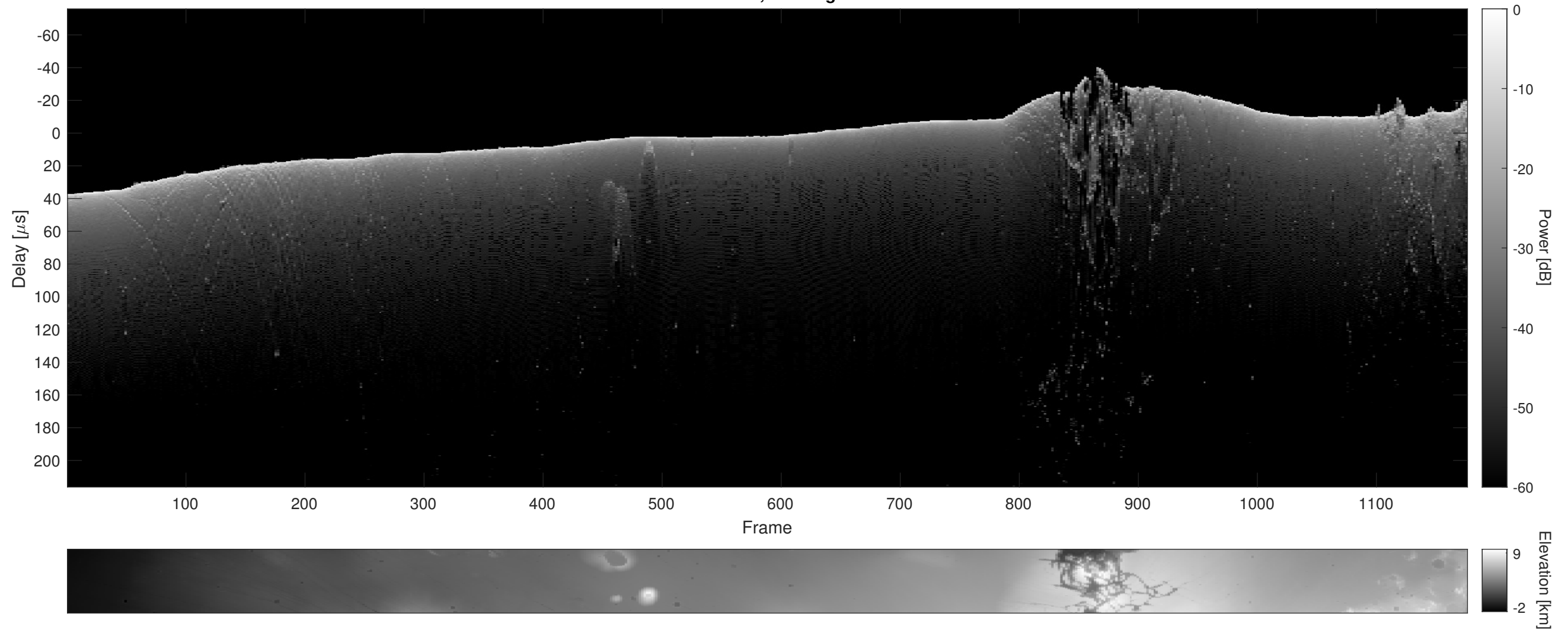
Orbit 15630, Cluttergram
