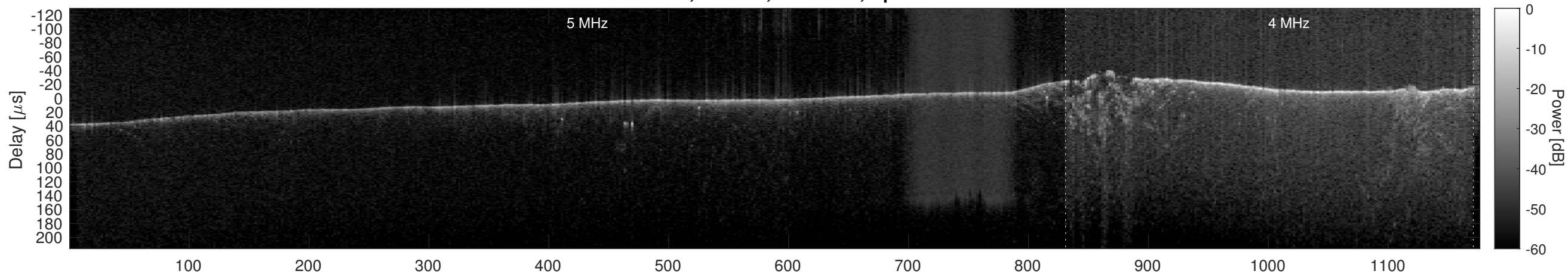
Orbit 15630, Cluttergram
