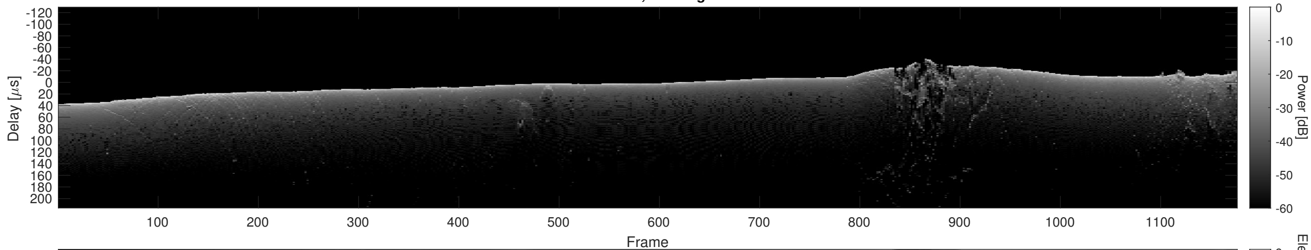
Orbit 15630, Cluttergram
