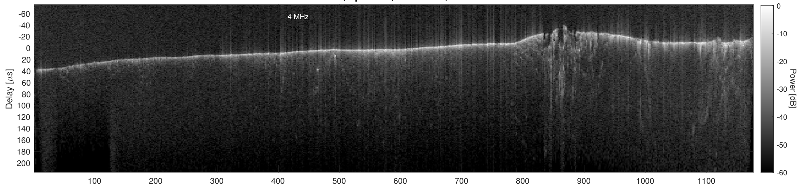
Orbit 15630, Cluttergram
