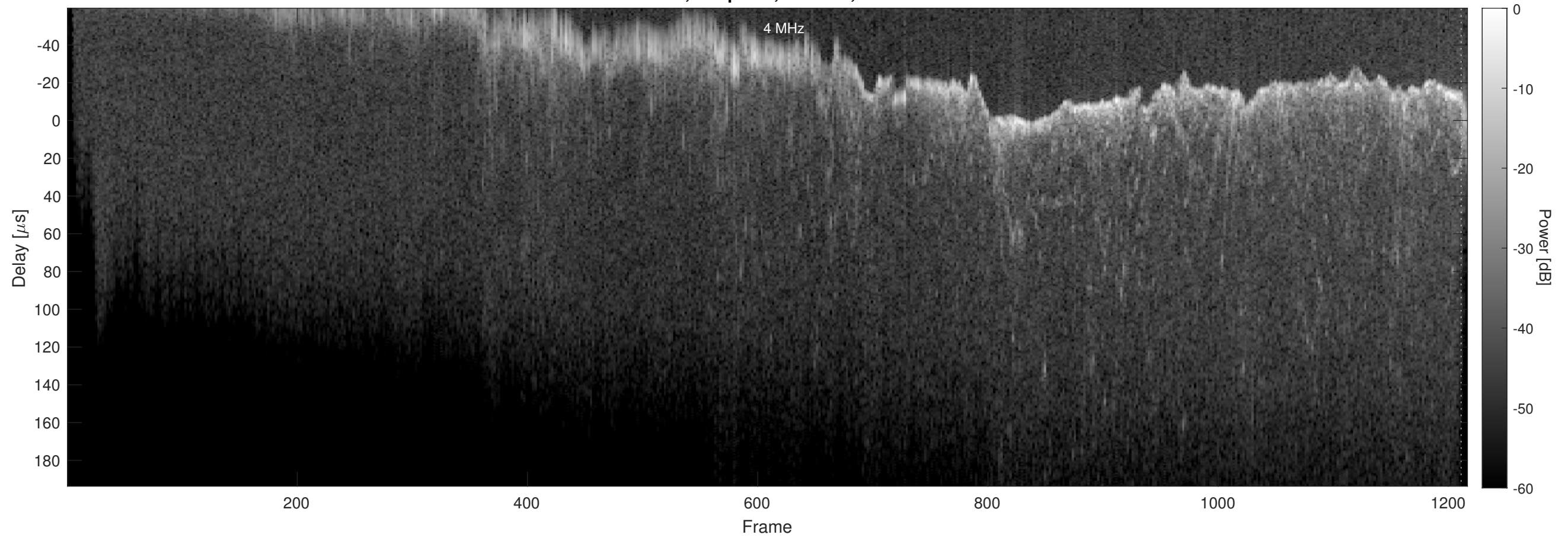
Orbit 15643, Chapman, Window, Channel 2
