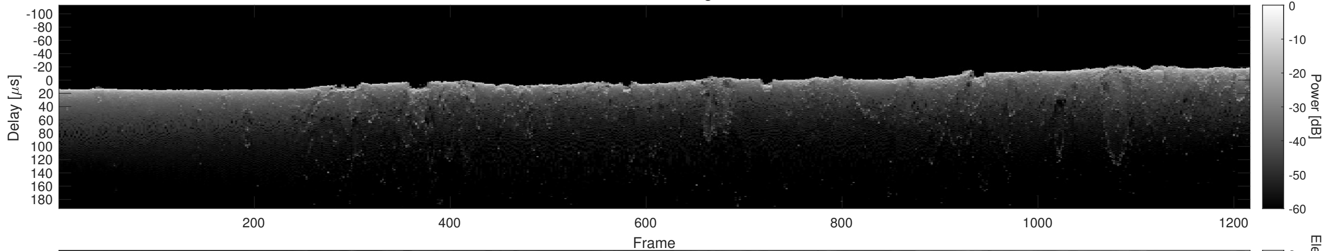
Orbit 15643, Cluttergram
