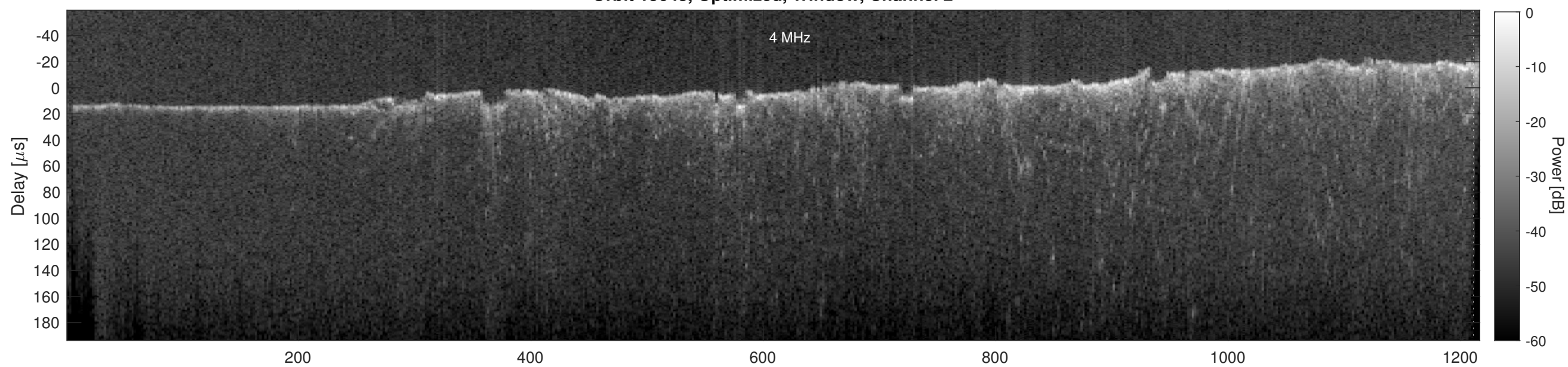
Orbit 15643, Cluttergram
