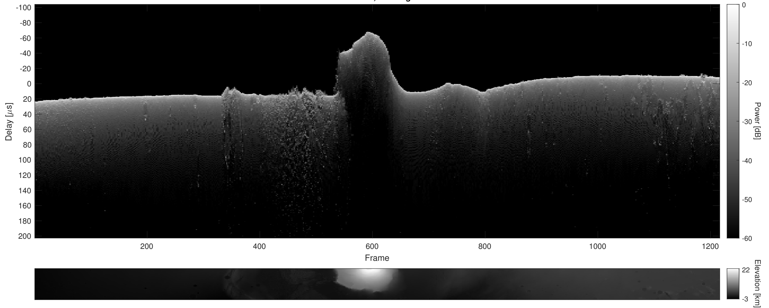
Orbit 15648, Cluttergram
