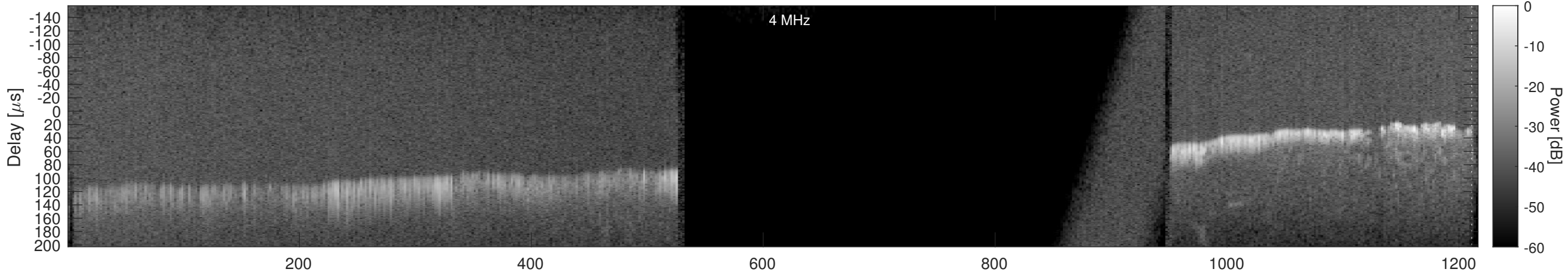
Orbit 15648, Window, Channel 2, Chapman
