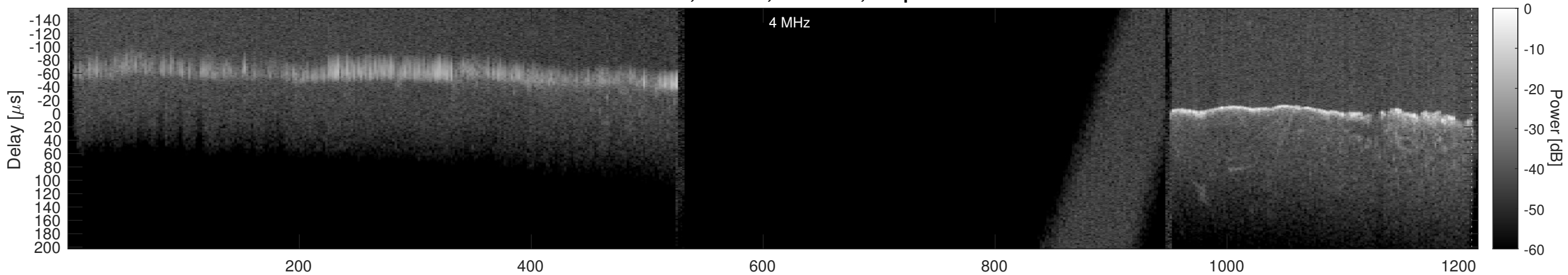
Orbit 15648, Window, Channel 2, Optimized
