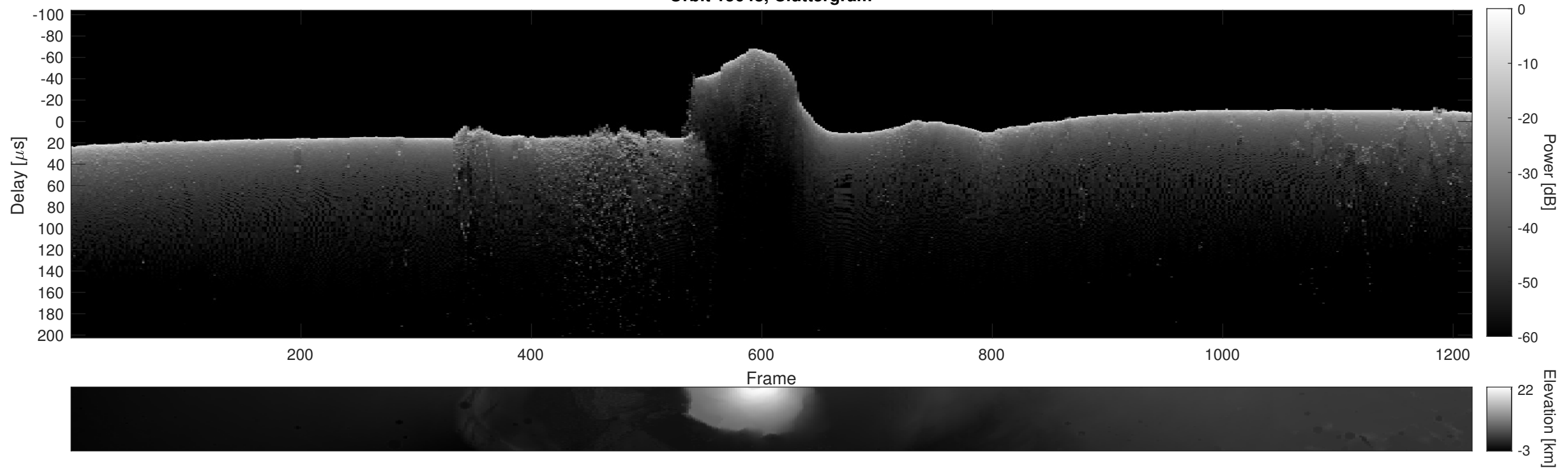
Orbit 15648, Cluttergram
