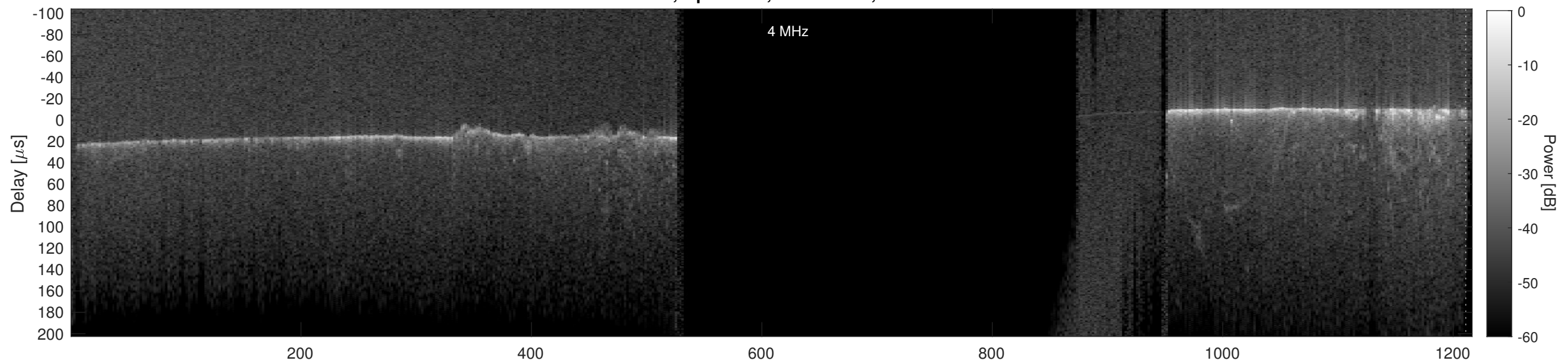
Orbit 15648, Cluttergram
