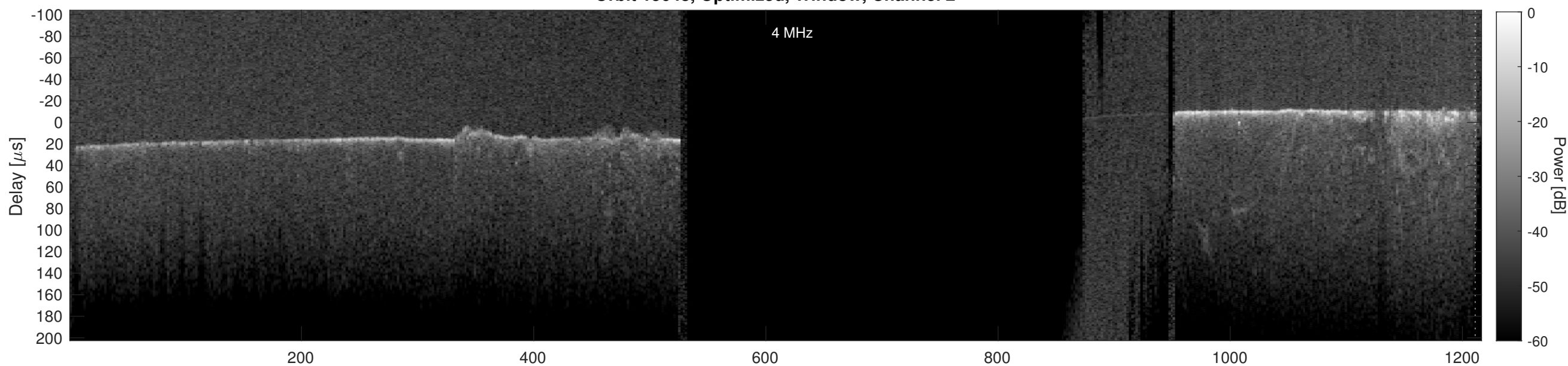
Orbit 15648, Cluttergram
