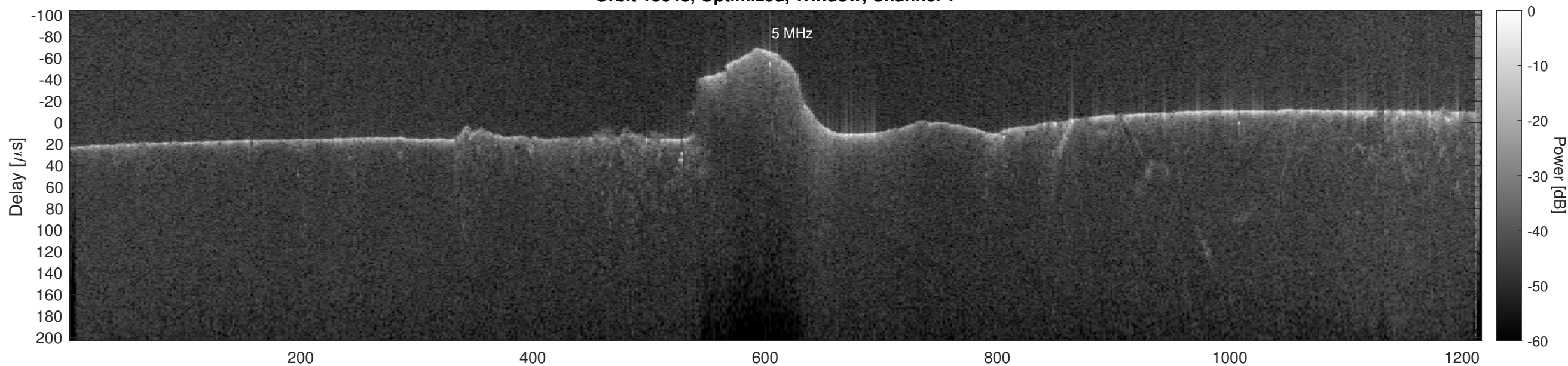
Orbit 15648, Optimized, Window, Channel 2
