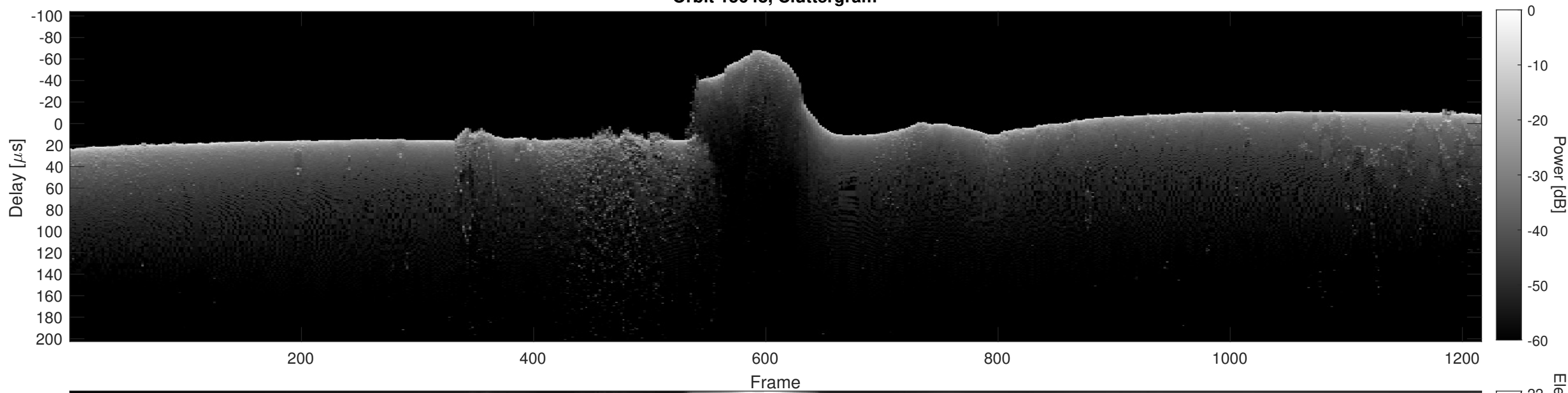
Orbit 15648, Cluttergram
