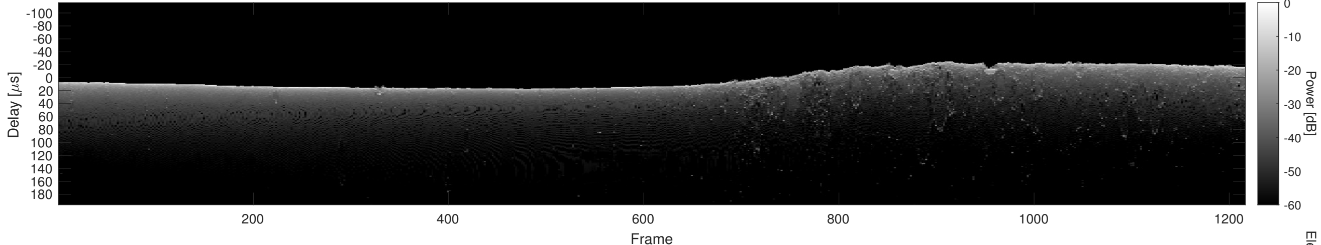
Orbit 15649, Cluttergram
