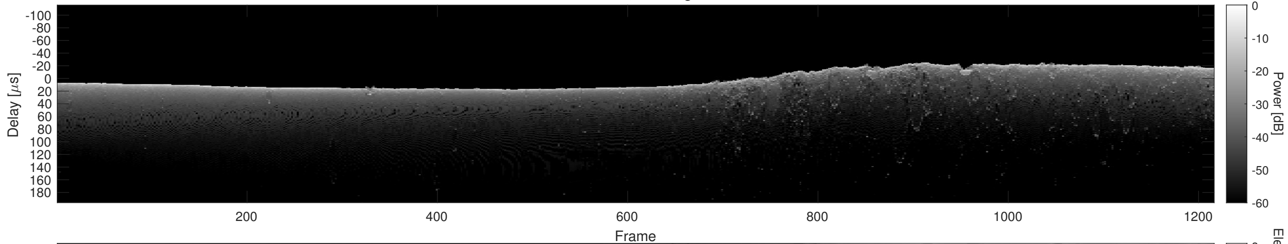
Orbit 15649, Cluttergram
