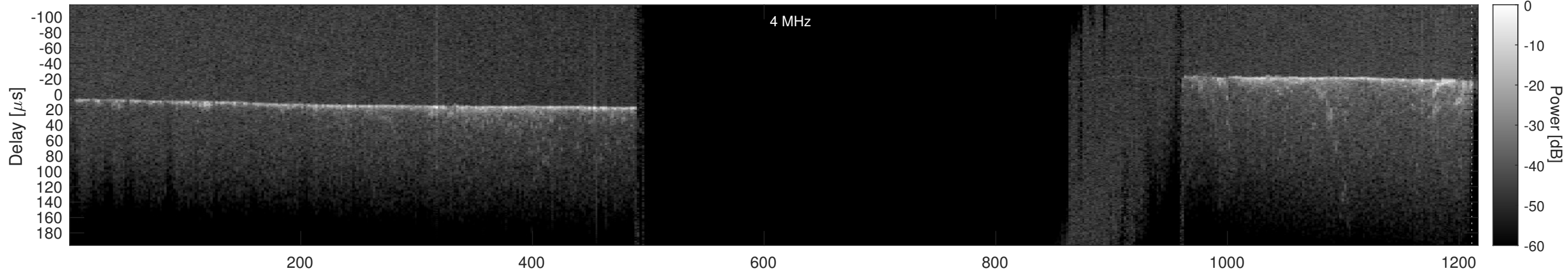
Orbit 15649, Cluttergram
