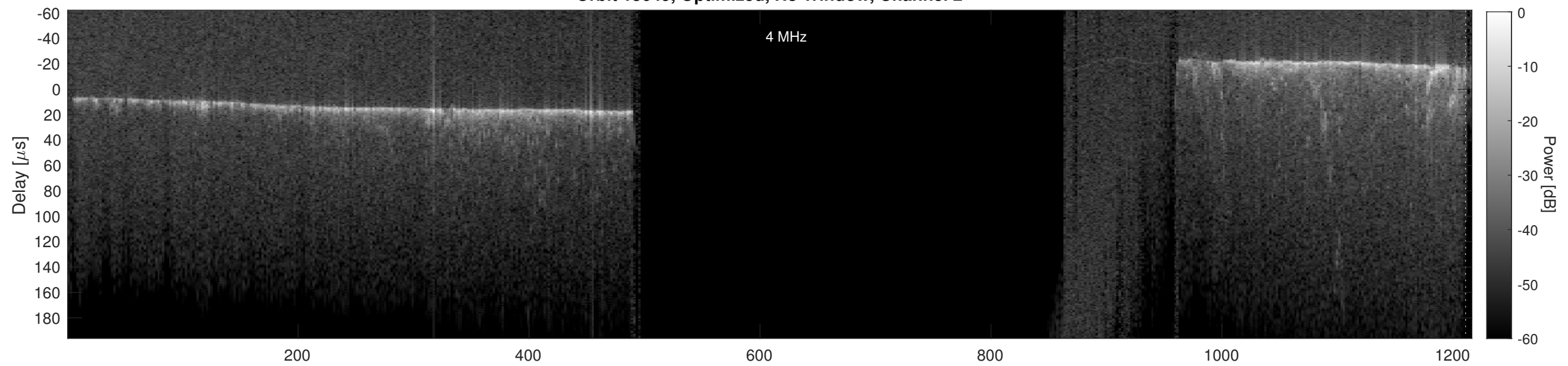
Orbit 15649, Cluttergram
