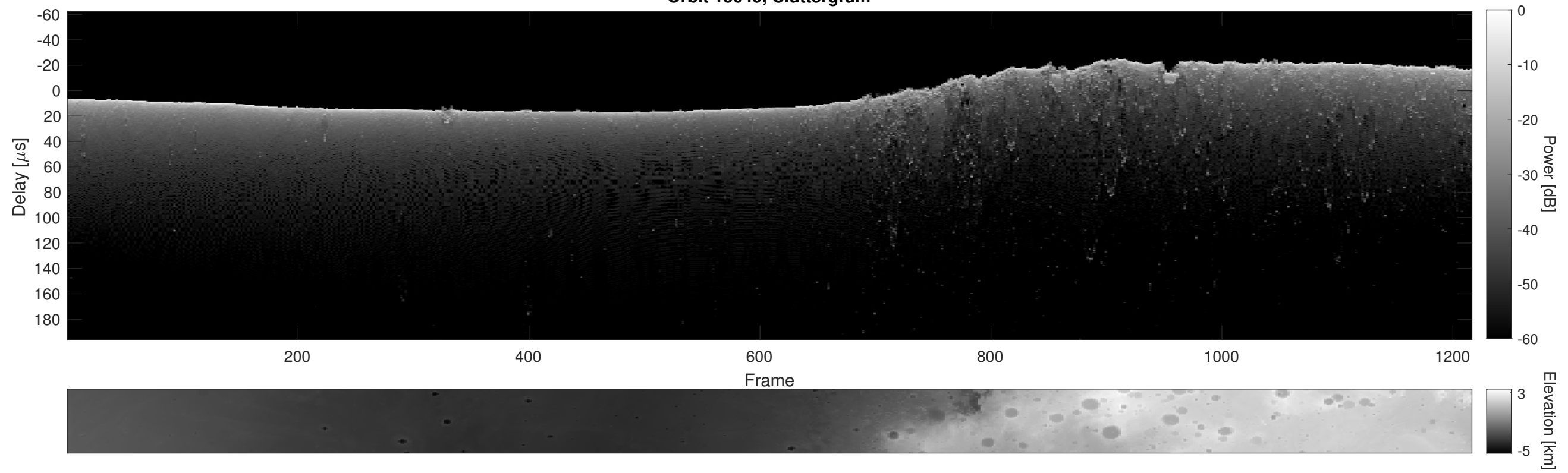
Orbit 15649, Cluttergram
