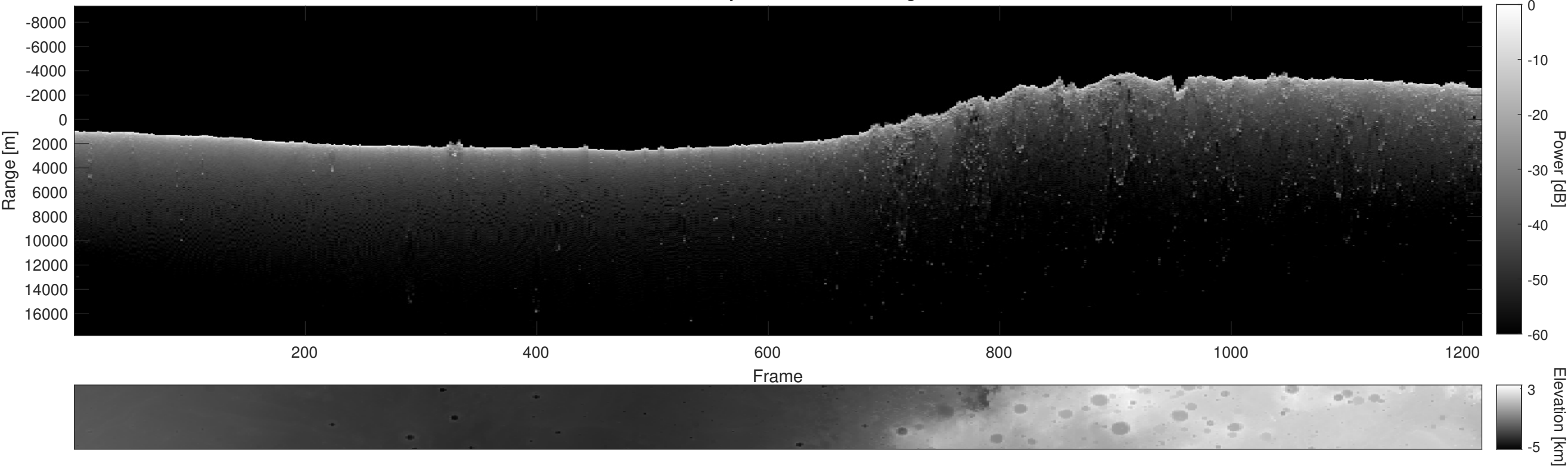
Orbit 15649, Depth-Corrected Cluttergram
