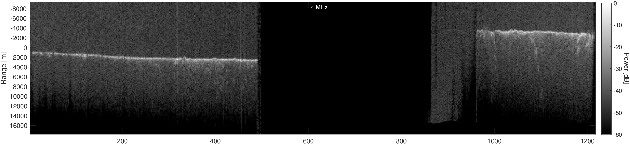
Orbit 15649, Depth-Corrected Cluttergram
