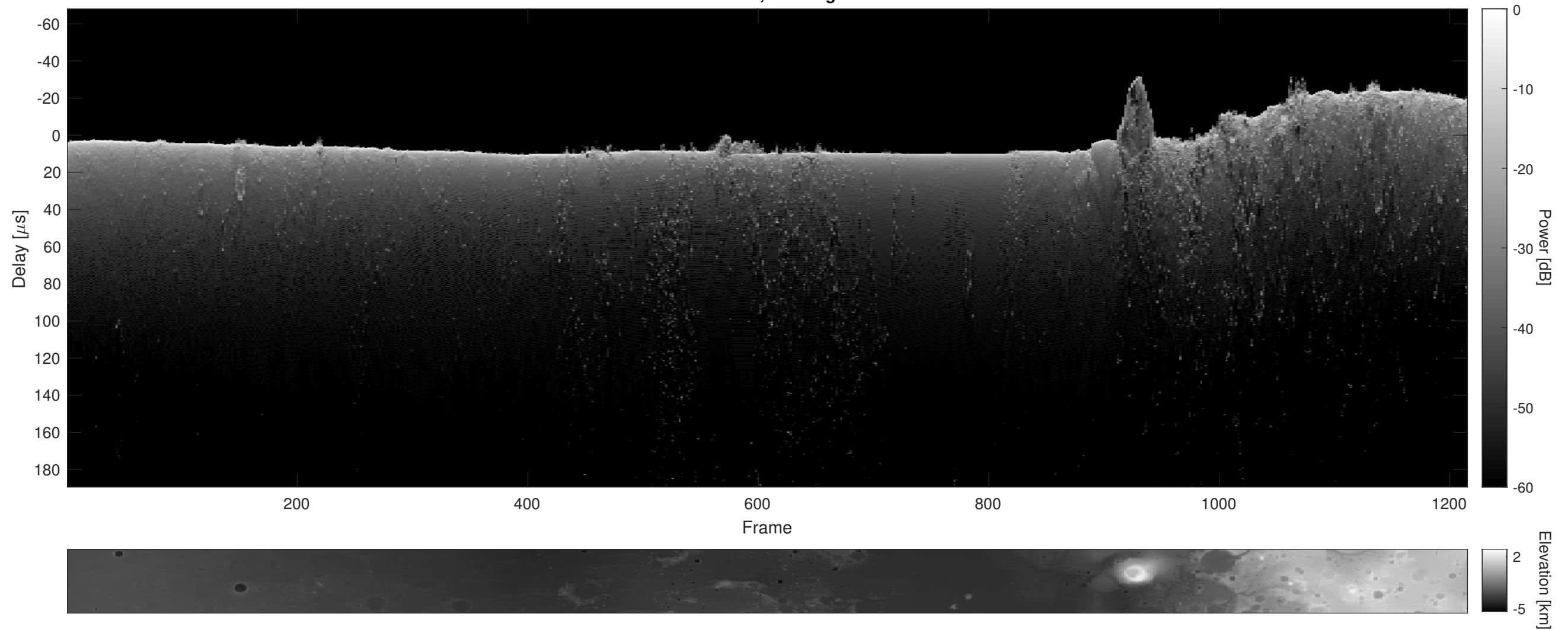
Orbit 15652, Cluttergram
