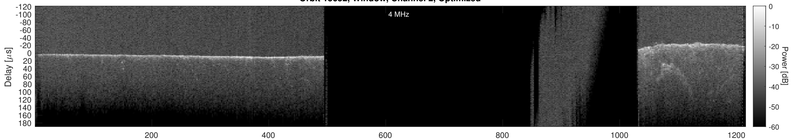
Orbit 15652, Cluttergram
