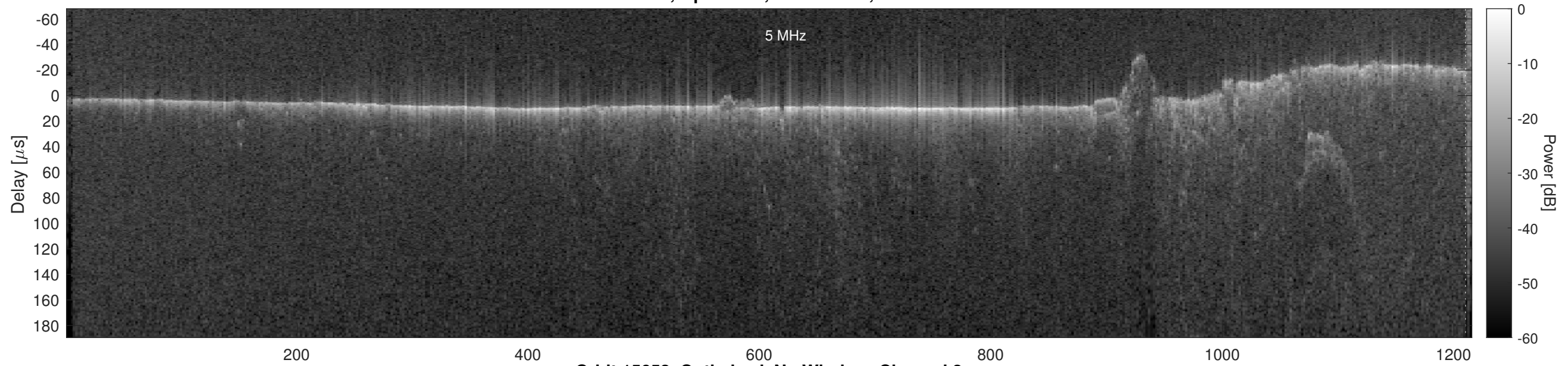
Orbit 15652, Optimized, No Window, Channel 2
