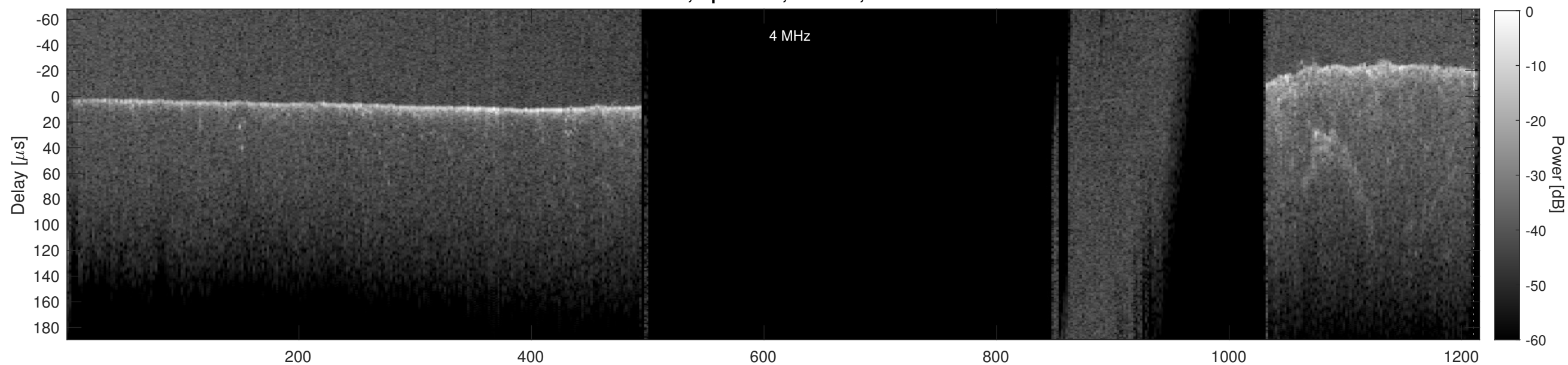
Orbit 15652, Cluttergram
