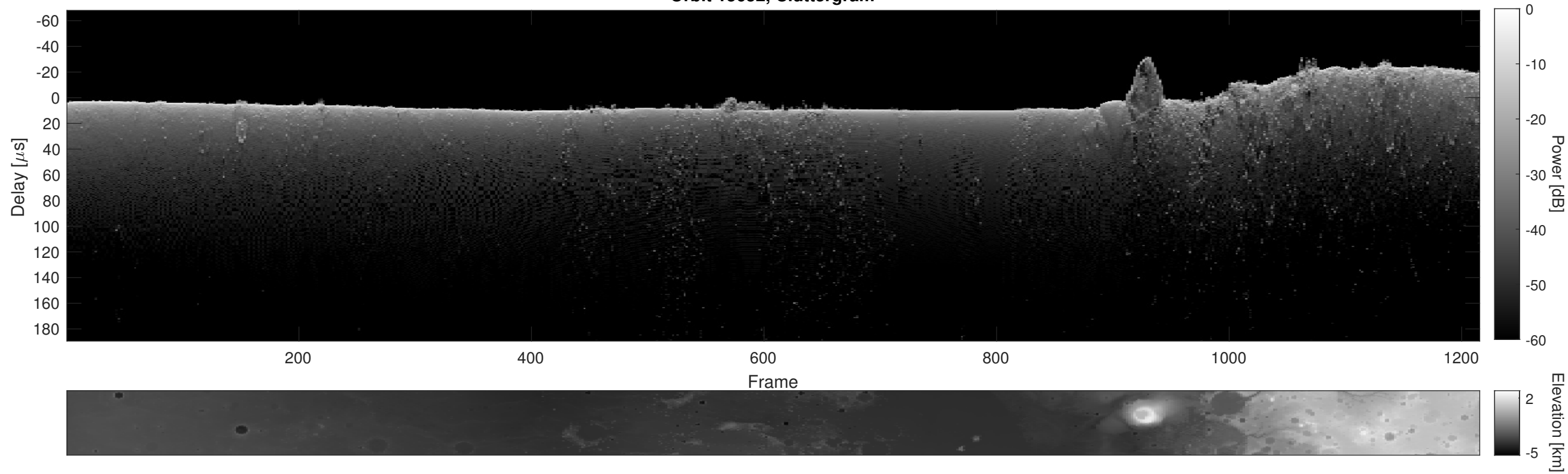
Orbit 15652, Cluttergram
