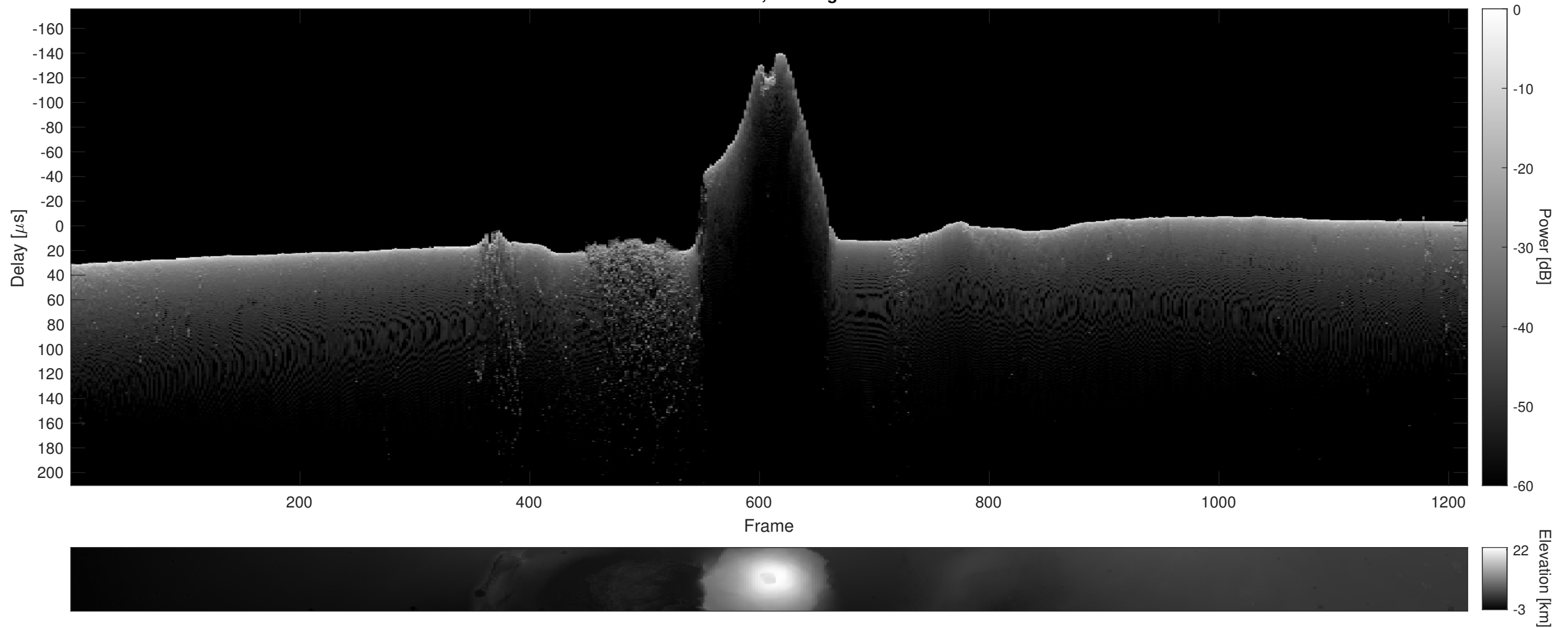
Orbit 15655, Cluttergram
