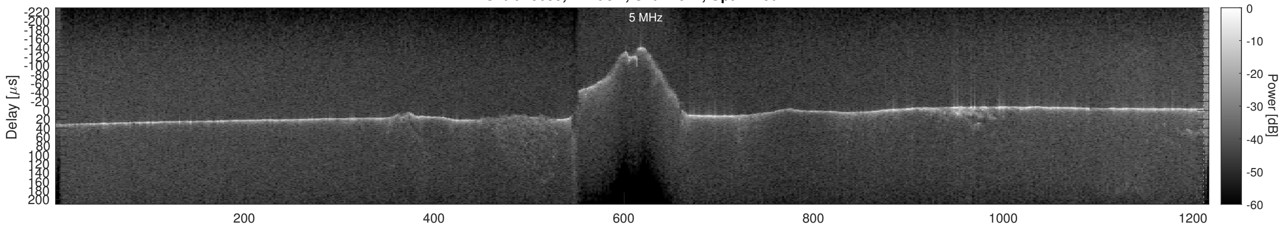
Orbit 15655, Cluttergram
