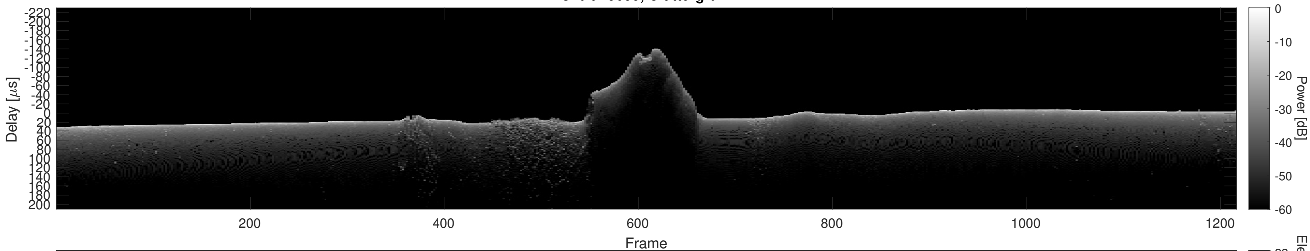
Orbit 15655, Cluttergram
