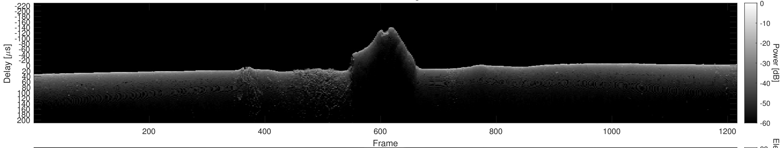
Orbit 15655, Cluttergram
