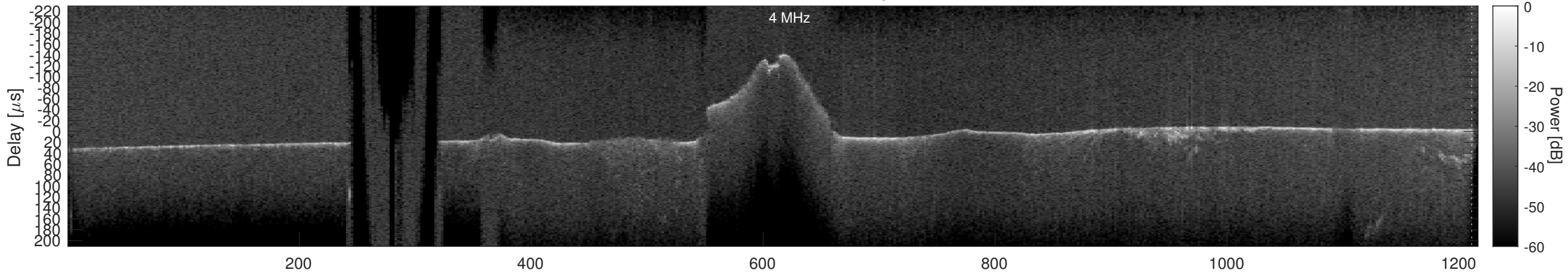
Orbit 15655, Cluttergram
