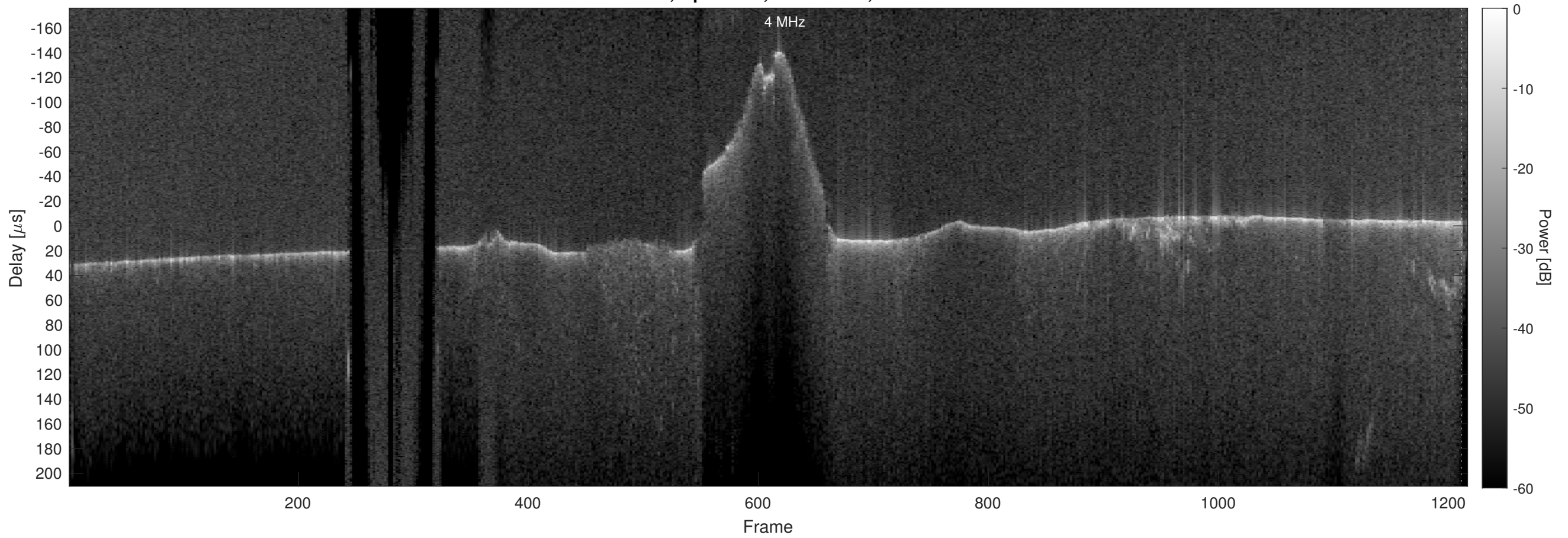
Orbit 15655, Optimized, No Window, Channel 2
