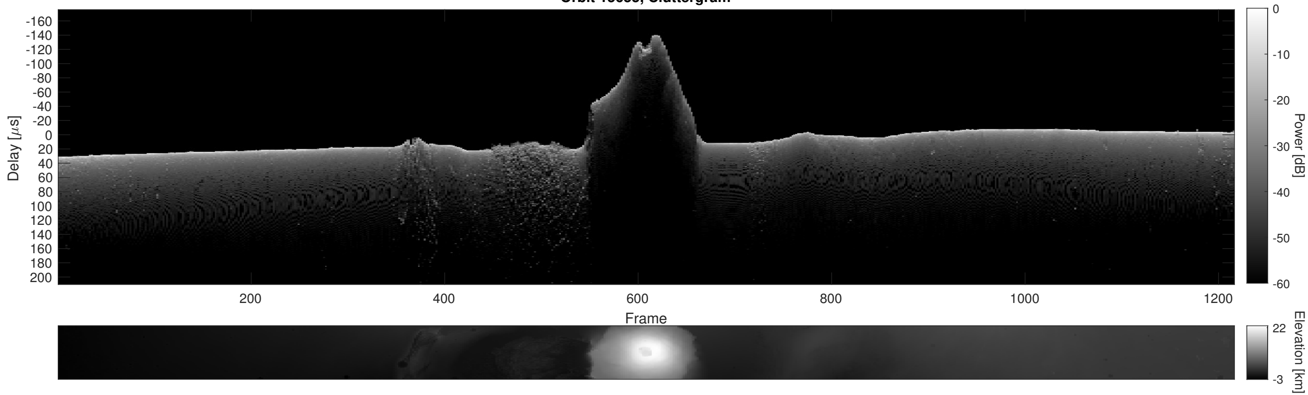
Orbit 15655, Cluttergram
