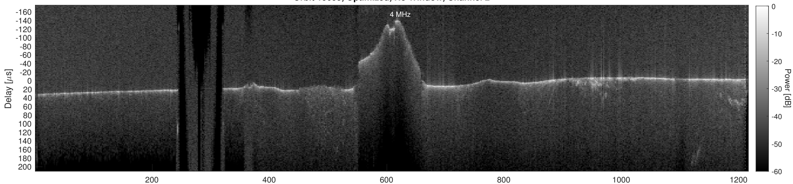
Orbit 15655, Cluttergram
