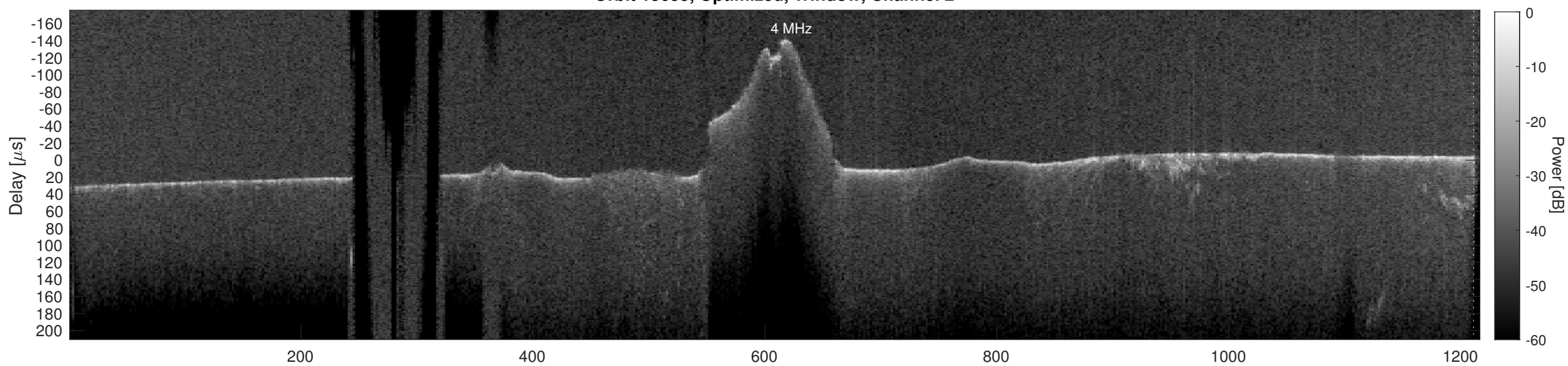
Orbit 15655, Cluttergram
