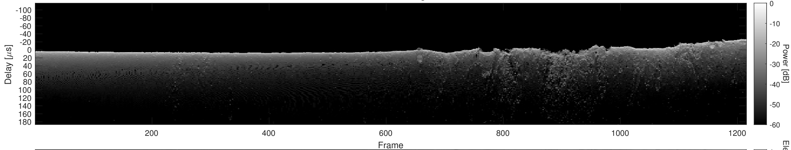
Orbit 15661, Cluttergram
