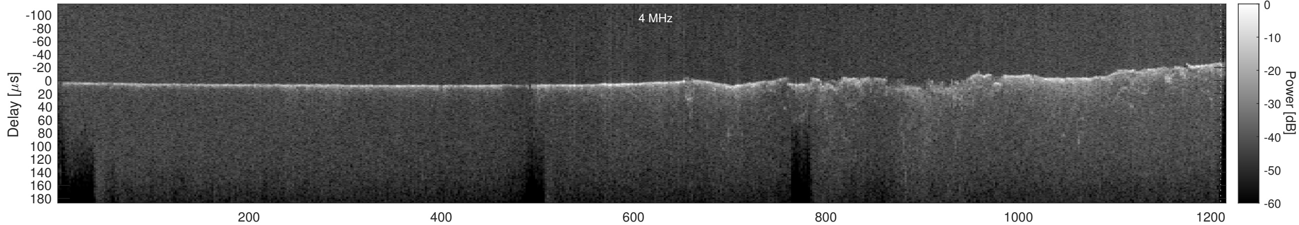
Orbit 15661, Cluttergram
