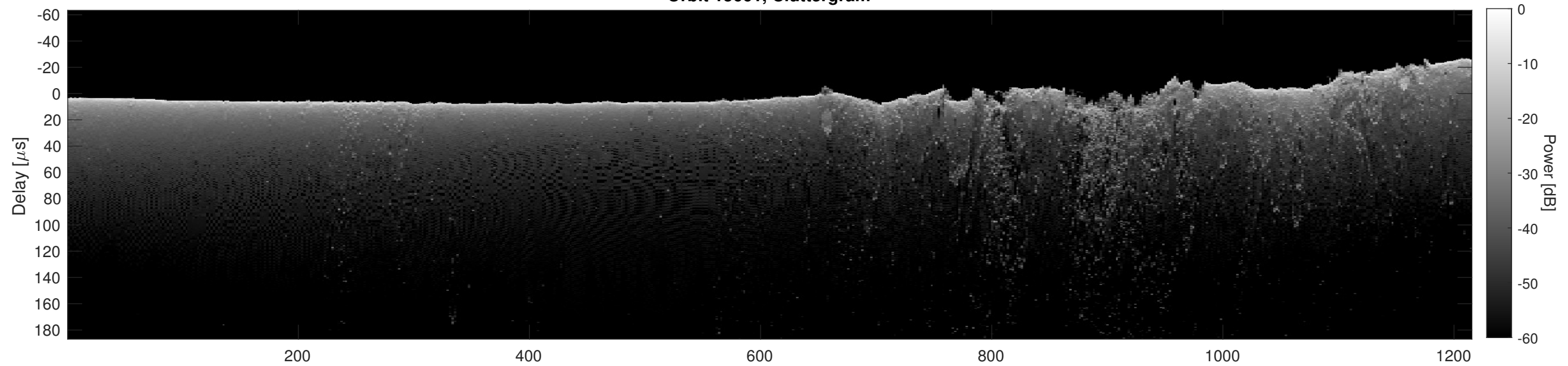
Orbit 15661, Cluttergram
