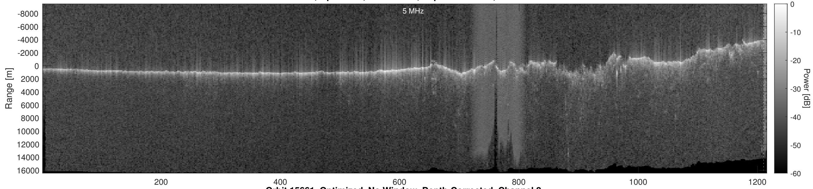
Orbit 15661, Optimized, No Window, Depth-Corrected, Channel 2
