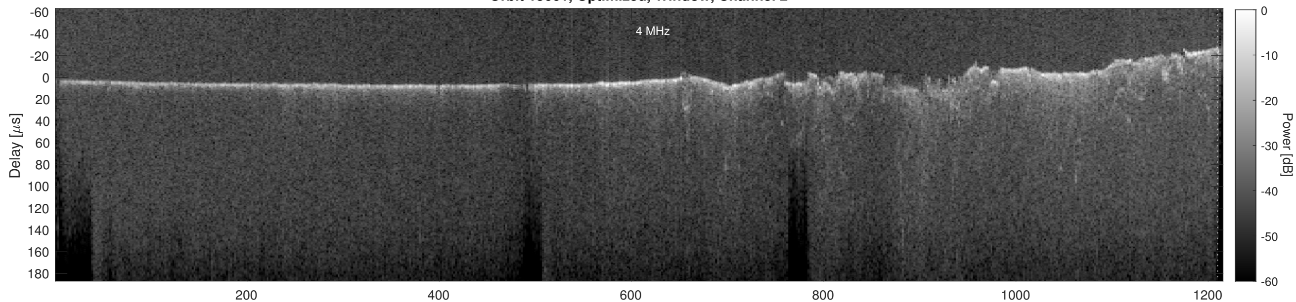
Orbit 15661, Cluttergram
