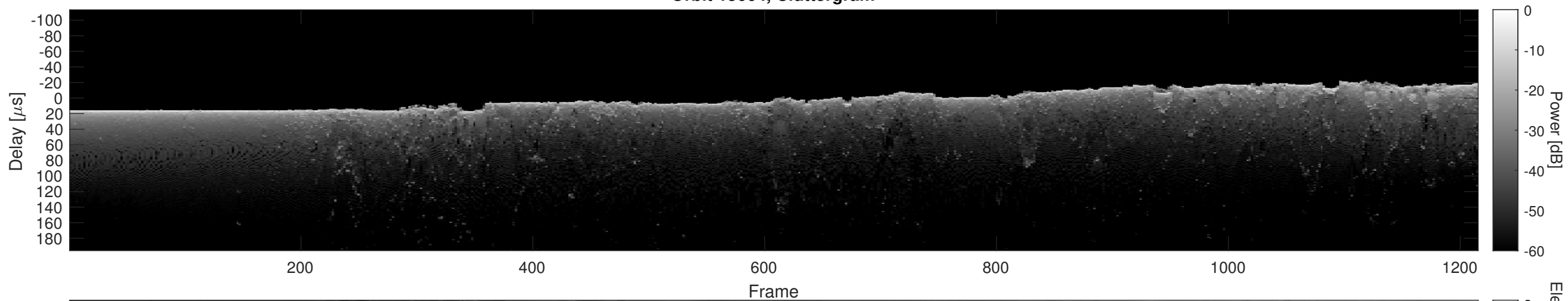
Orbit 15664, Cluttergram
