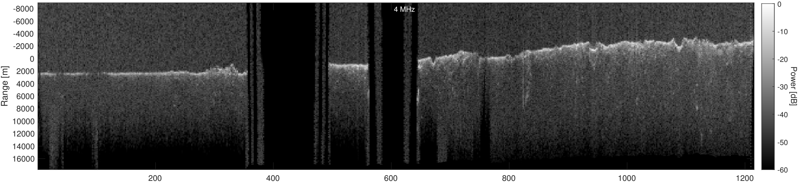
Orbit 15664, Depth-Corrected Cluttergram
