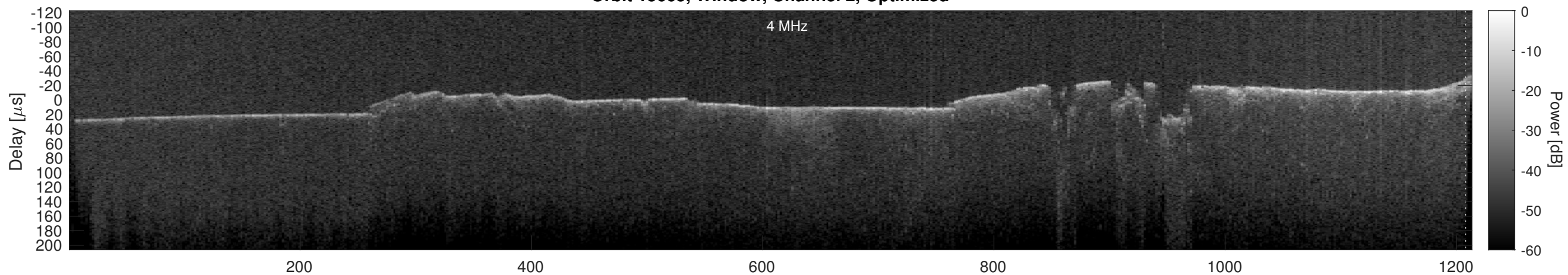
Orbit 15665, Cluttergram
