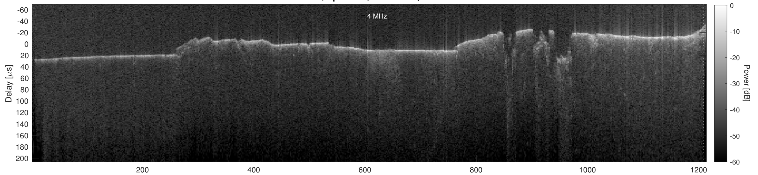
Orbit 15665, Cluttergram
