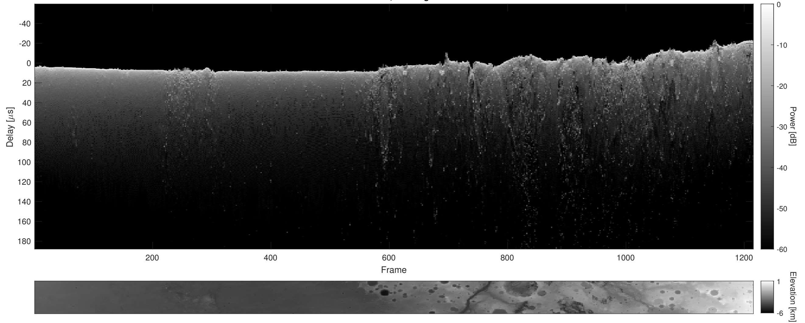
Orbit 15668, Cluttergram
