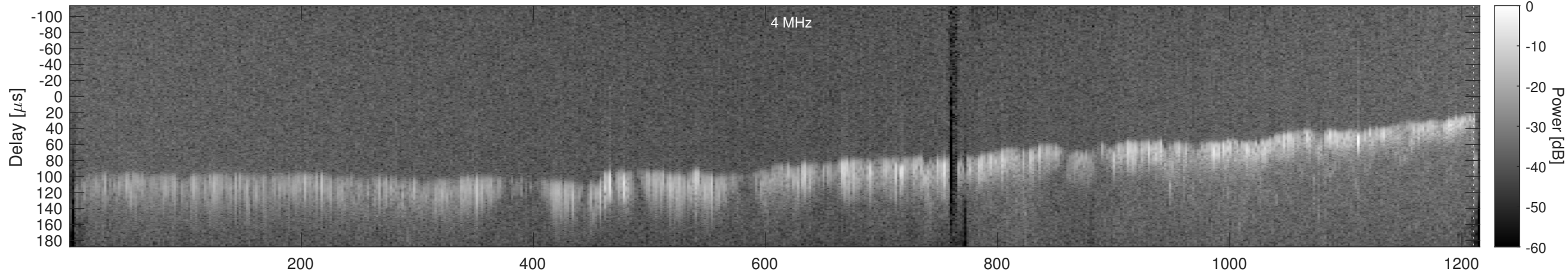
Orbit 15668, Window, Channel 2, Chapman
