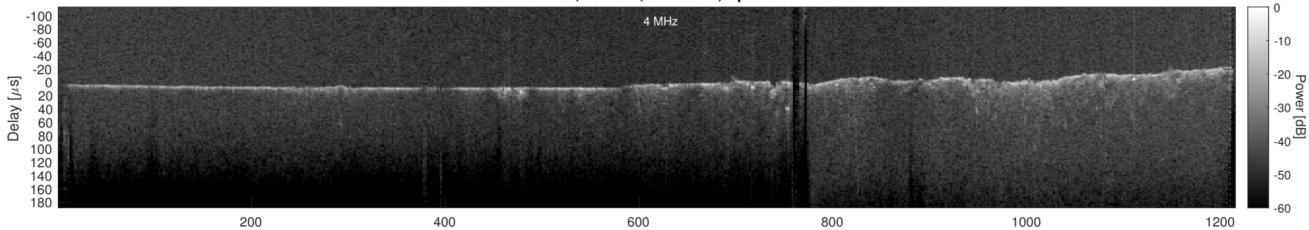
Orbit 15668, Cluttergram
