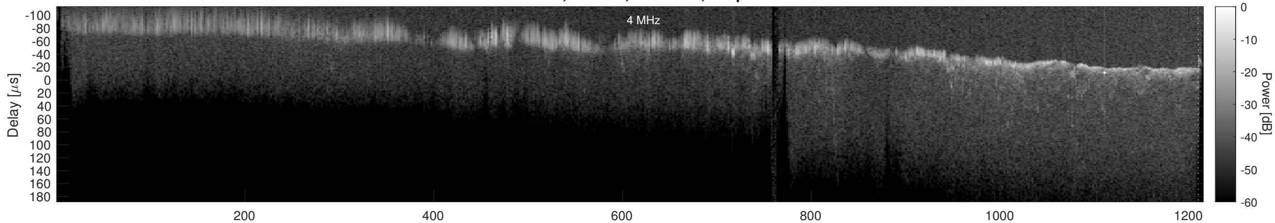
Orbit 15668, Window, Channel 2, Optimized
