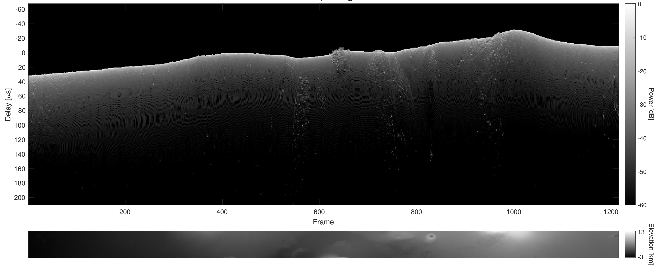
Orbit 15669, Cluttergram
