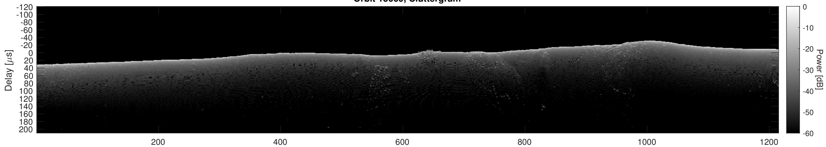
Orbit 15669, Cluttergram
