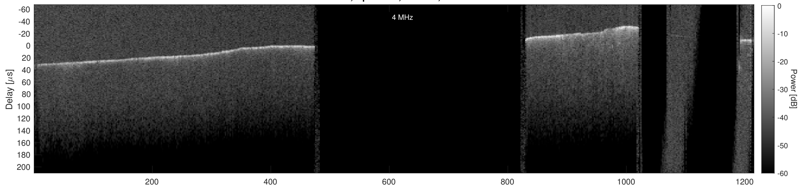
Orbit 15669, Cluttergram
