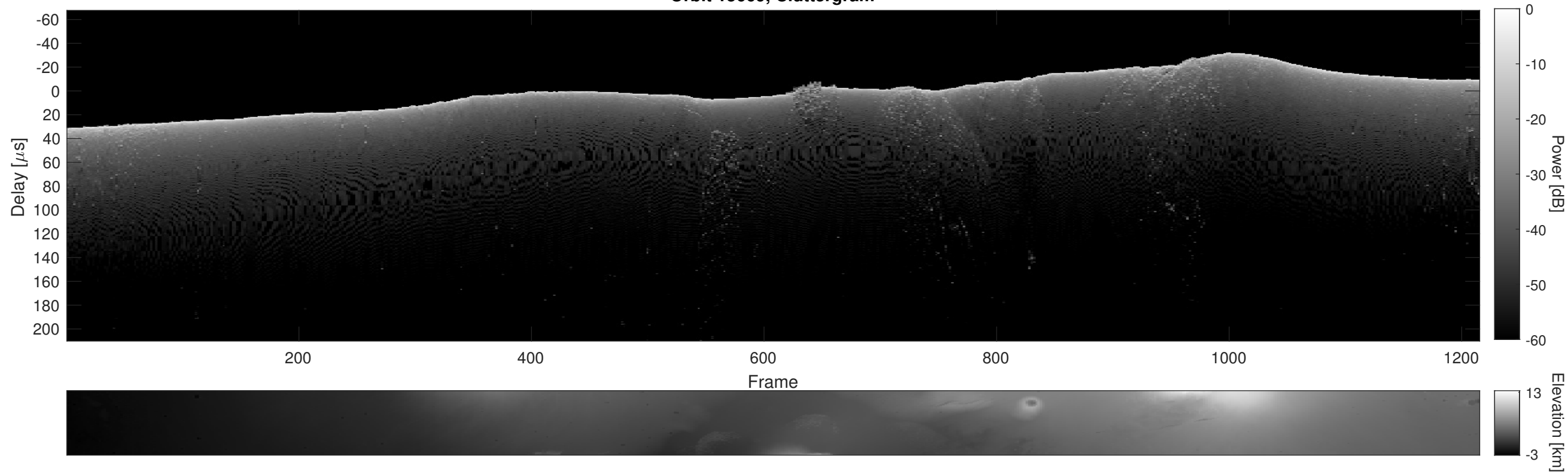
Orbit 15669, Cluttergram
