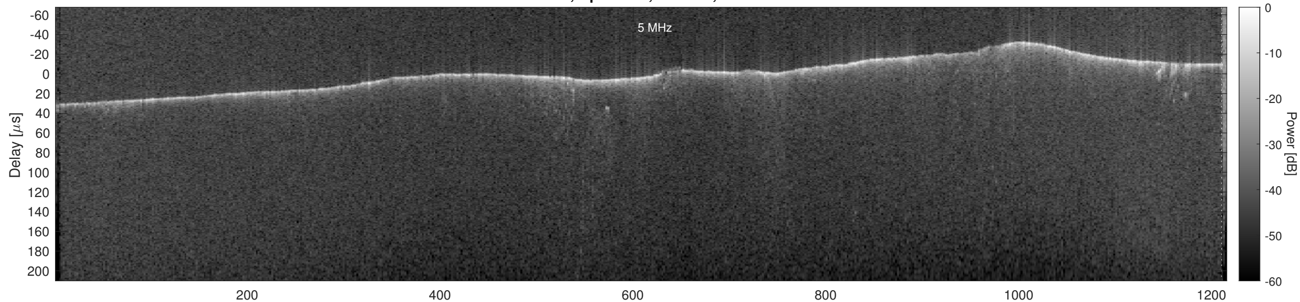
Orbit 15669, Optimized, Window, Channel 2
