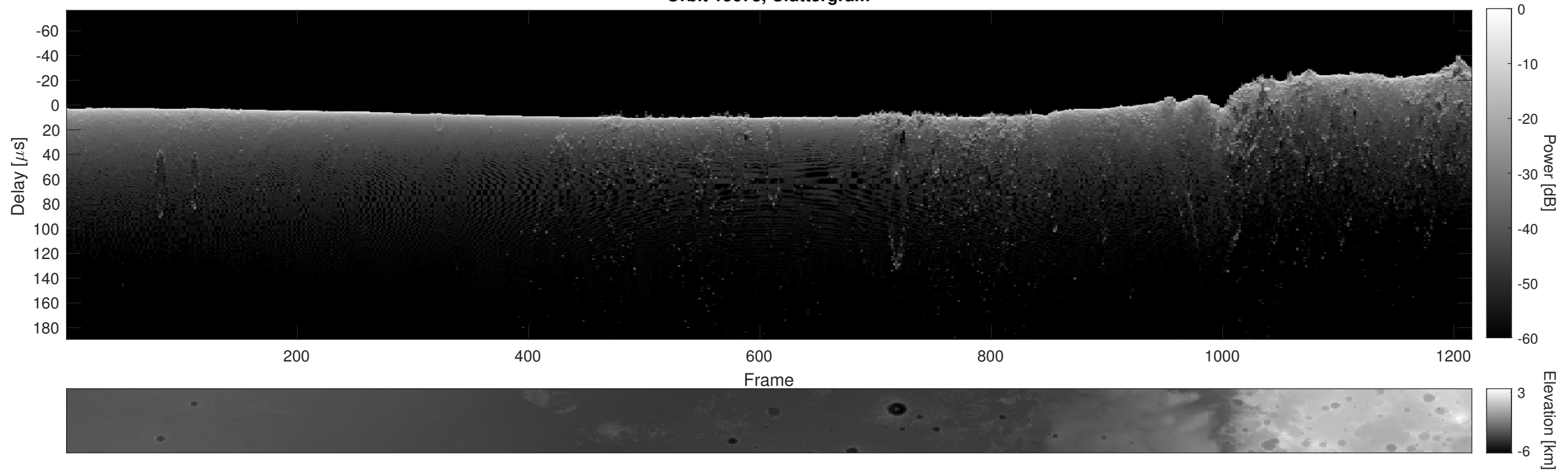
Orbit 15673, Cluttergram
