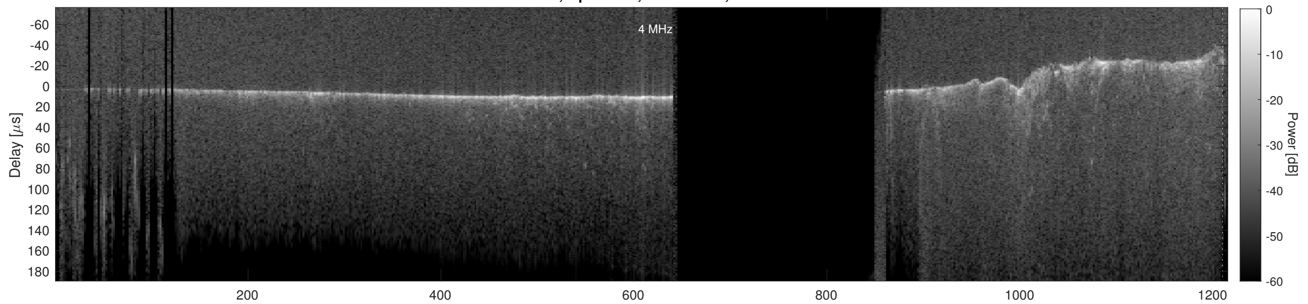
Orbit 15673, Cluttergram
